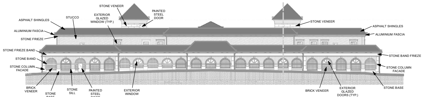
EAST ELEVATION
