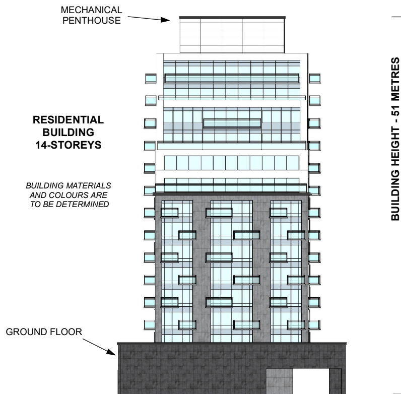
NORTH ELEVATION - FACING ARROWHEAD DRIVE
