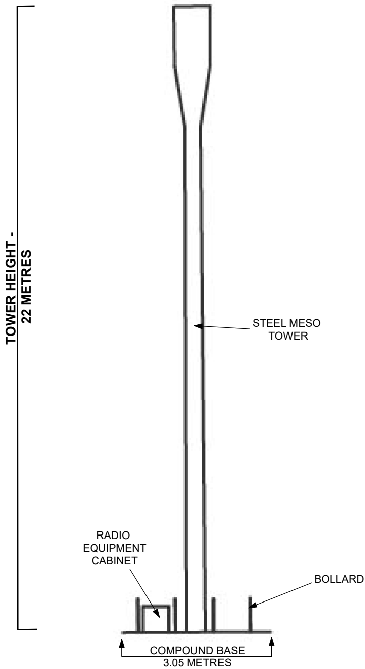
South Elevation
