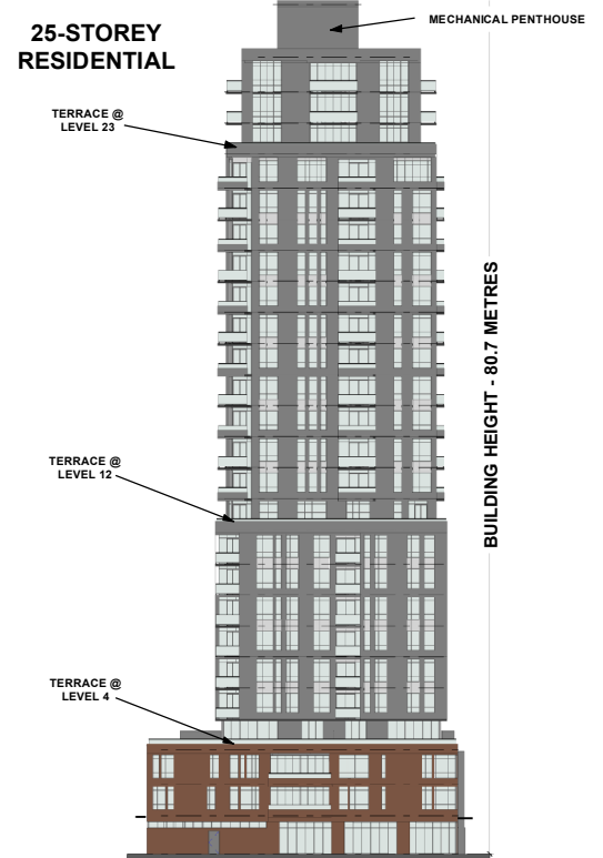
WEST ELEVATION
