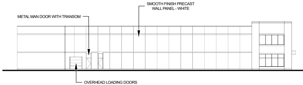
WEST ELEVATION
