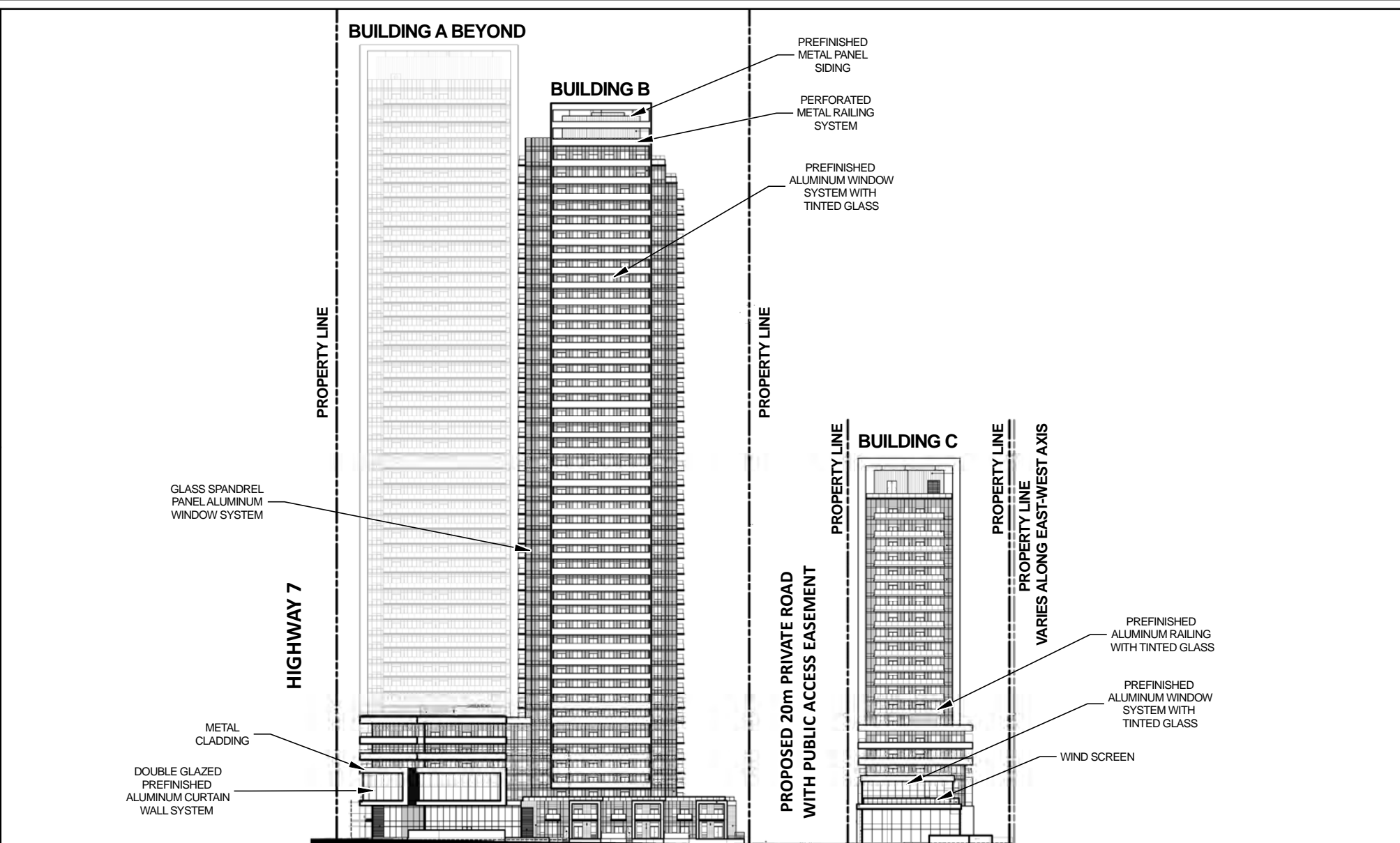
WEST ELEVATION - FACING MAPLECRETE ROAD
