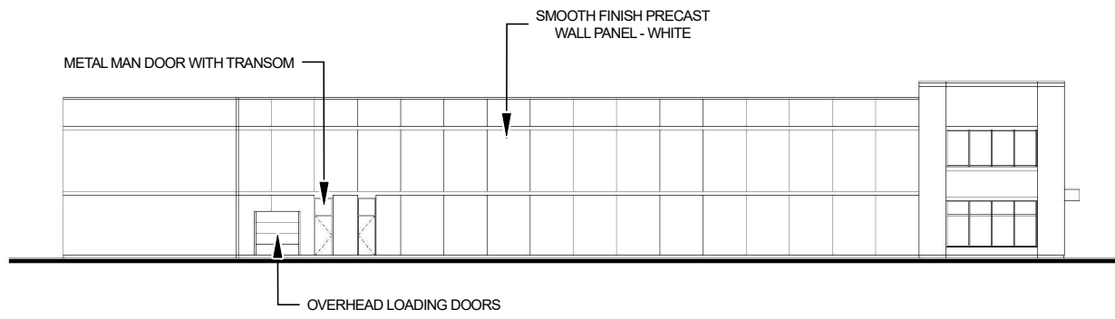
WEST ELEVATION
