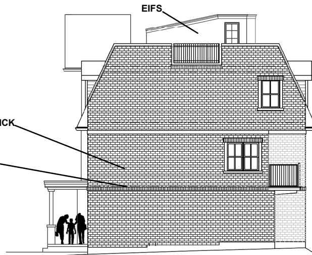
SOUTH ELEVATION
