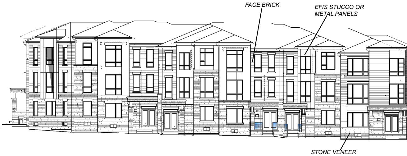
EAST (FRONT) ELEVATION - FACING BATHURST STREET
