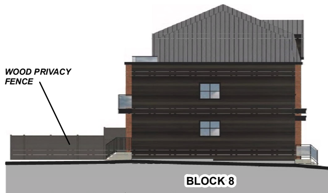
SOUTH ELEVATION
