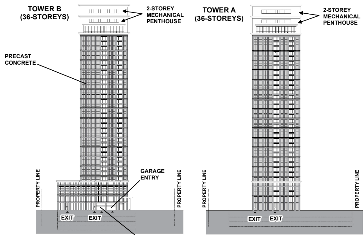
EAST ELEVATION
