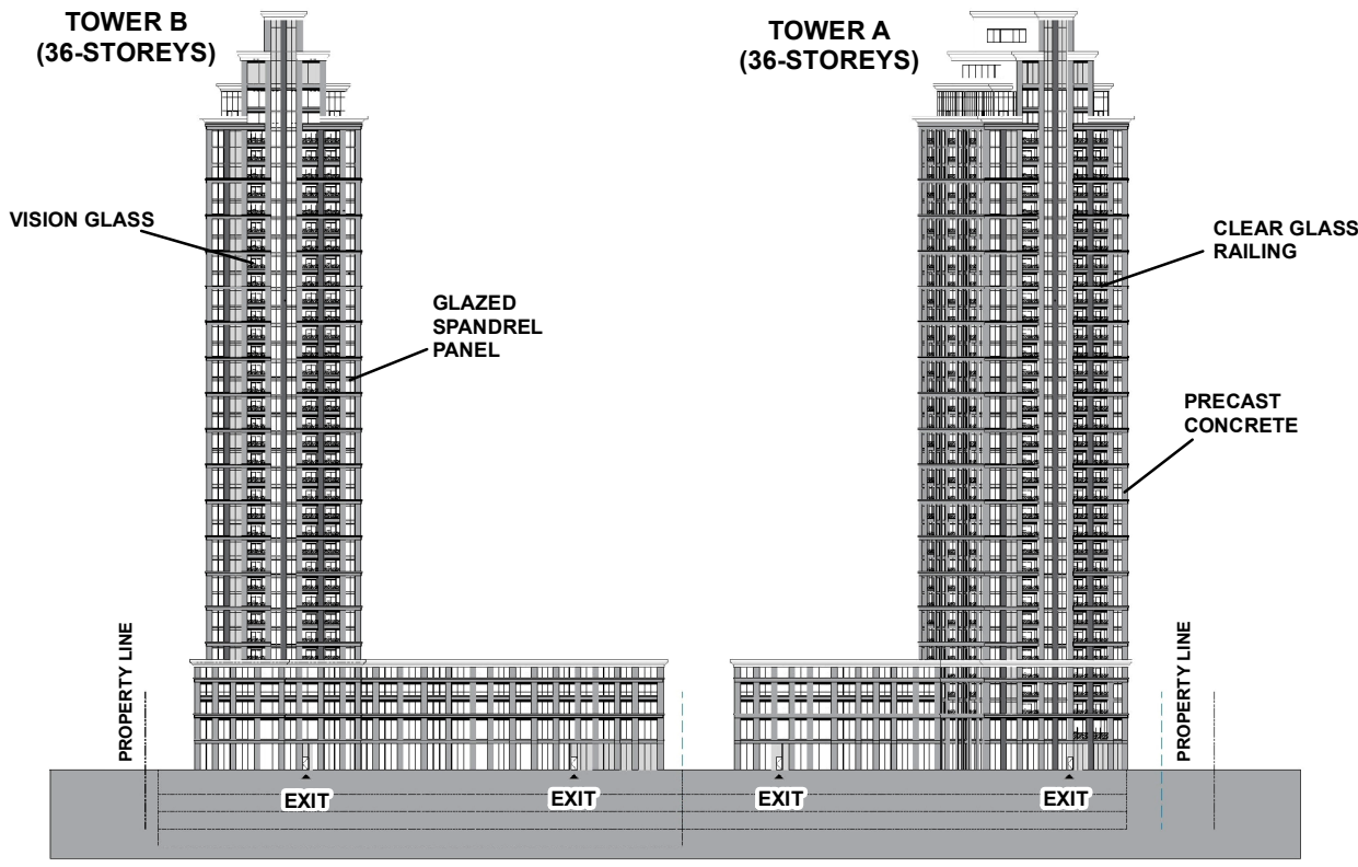
SOUTH ELEVATION
