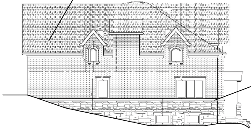
WEST ELEVATION
