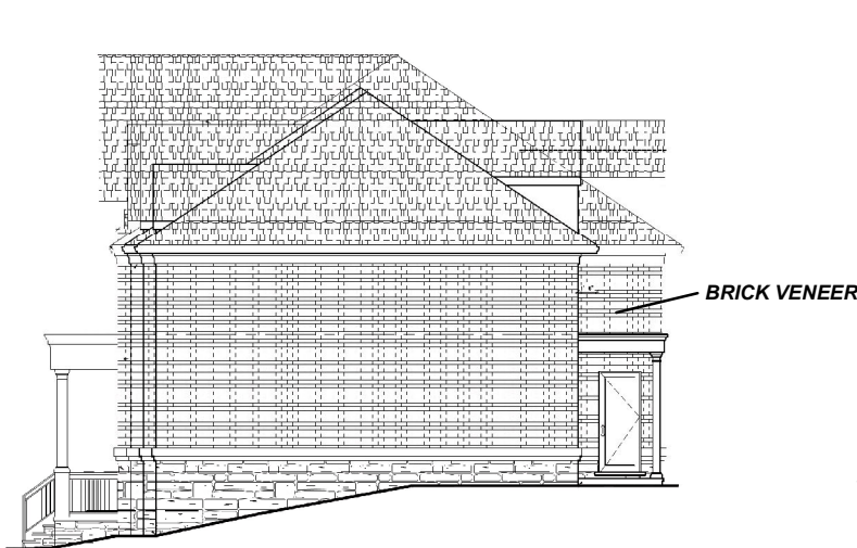
NORTH ELEVATION
