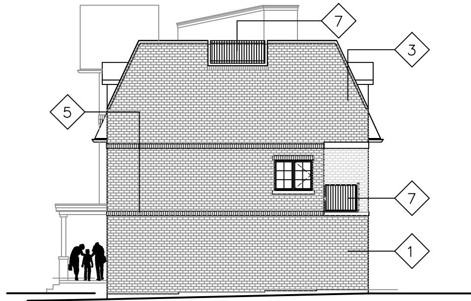
SOUTH ELEVATION
