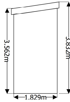
SHED SIDE VIEW
