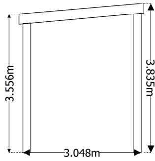
PERGOLA SIDE VIEW
