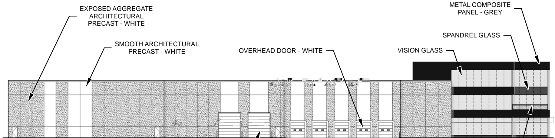
WEST (SIDE) ELEVATION
