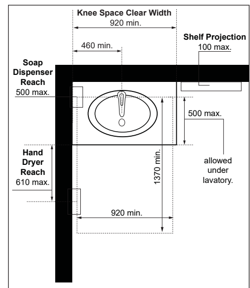
Figure 59b: Lavatories - Plan View
