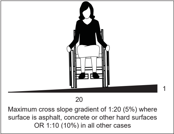
Figure 31b: Cross Slope
