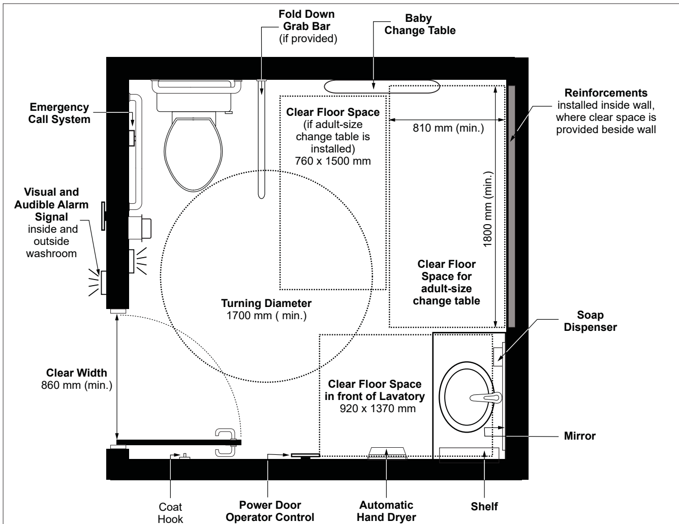
Figure 53: Universal Washroom
