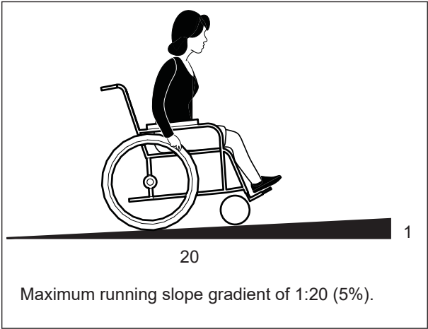
Figure 31a: Running Slope
