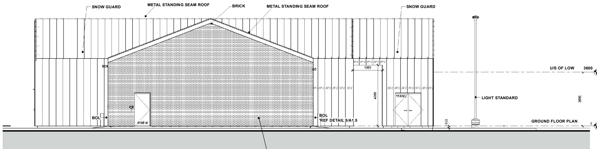
NORTH ELEVATION
