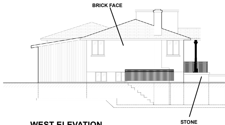
WEST ELEVATION
