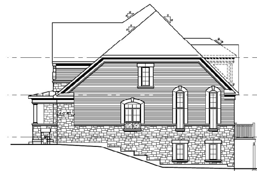
NORTH ELEVATION (LEFT)
