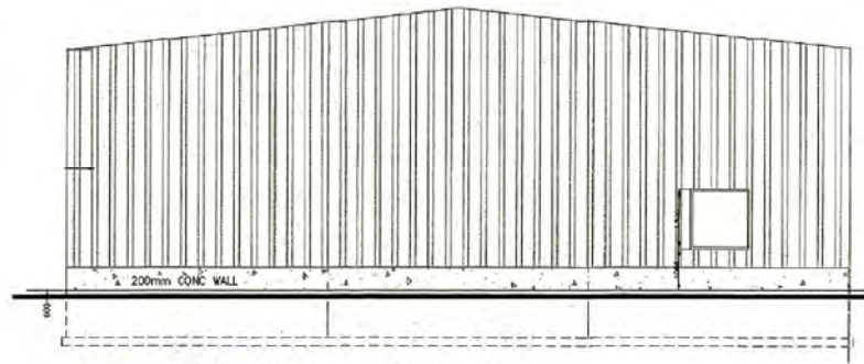
EAST ELEVATION (FACING KEELE STREET)
