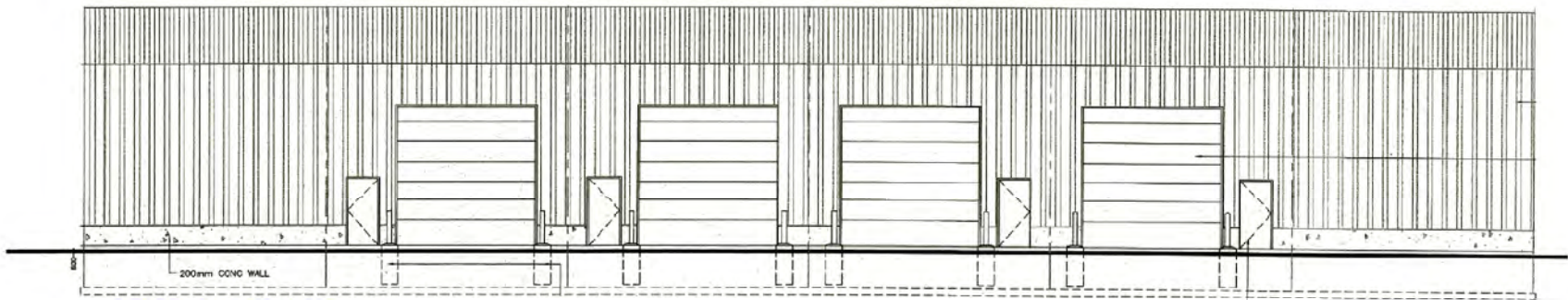
SOUTH ELEVATION
