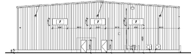
West Elevation
