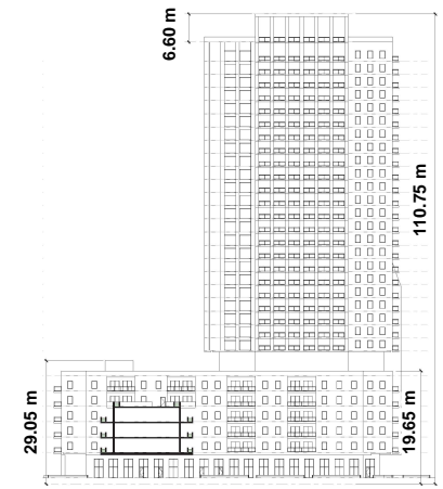
Building H - 30 Storeys Not to Scale
