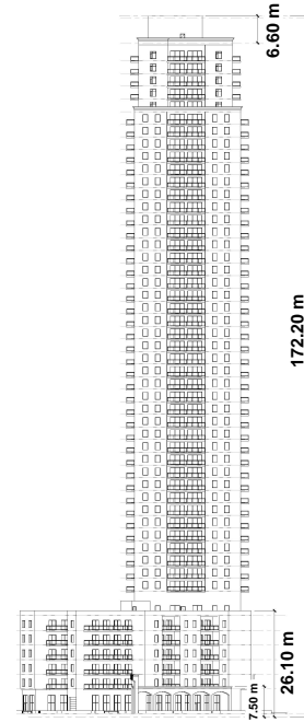
Building C - 50 Storeys
