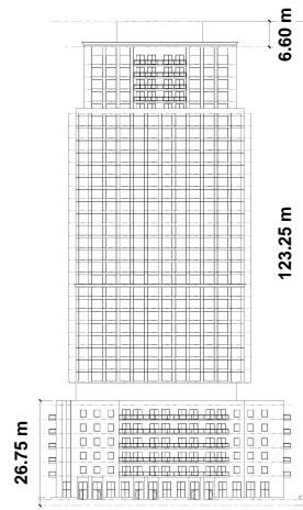
Building F - 34 Storeys
