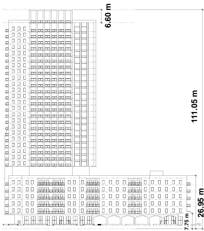
Building E - 30 Storeys
