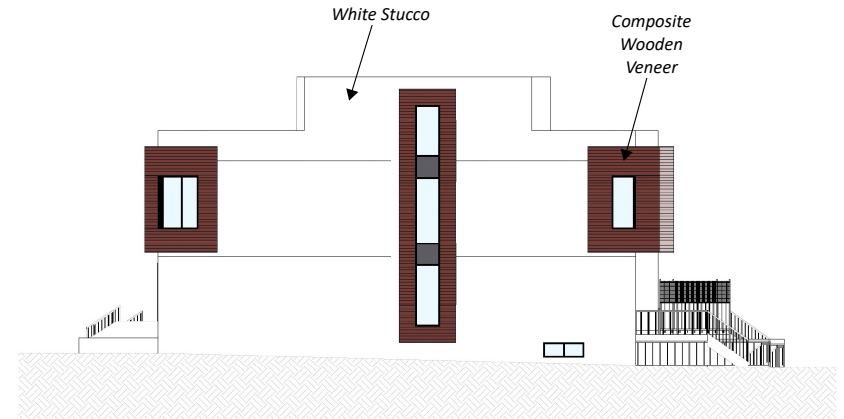
North Elevation
