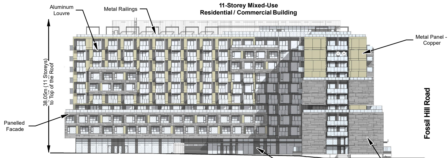
South Elevation (Facing Sibella Way)
