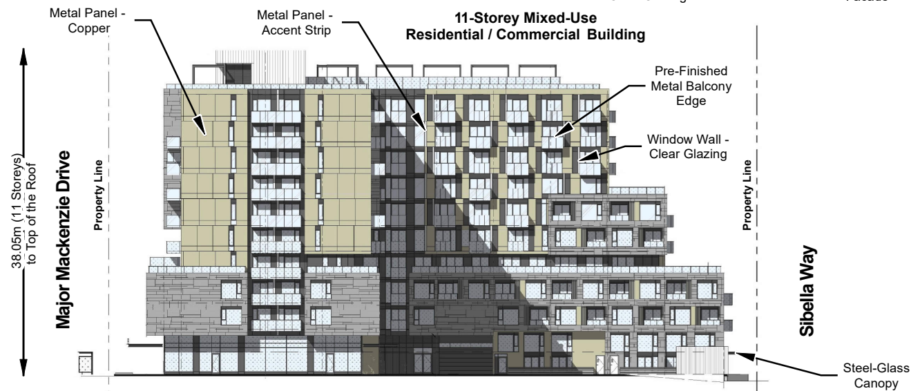
West Elevation
