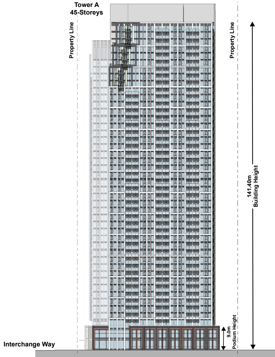
East Elevation - Facing Jane Street
