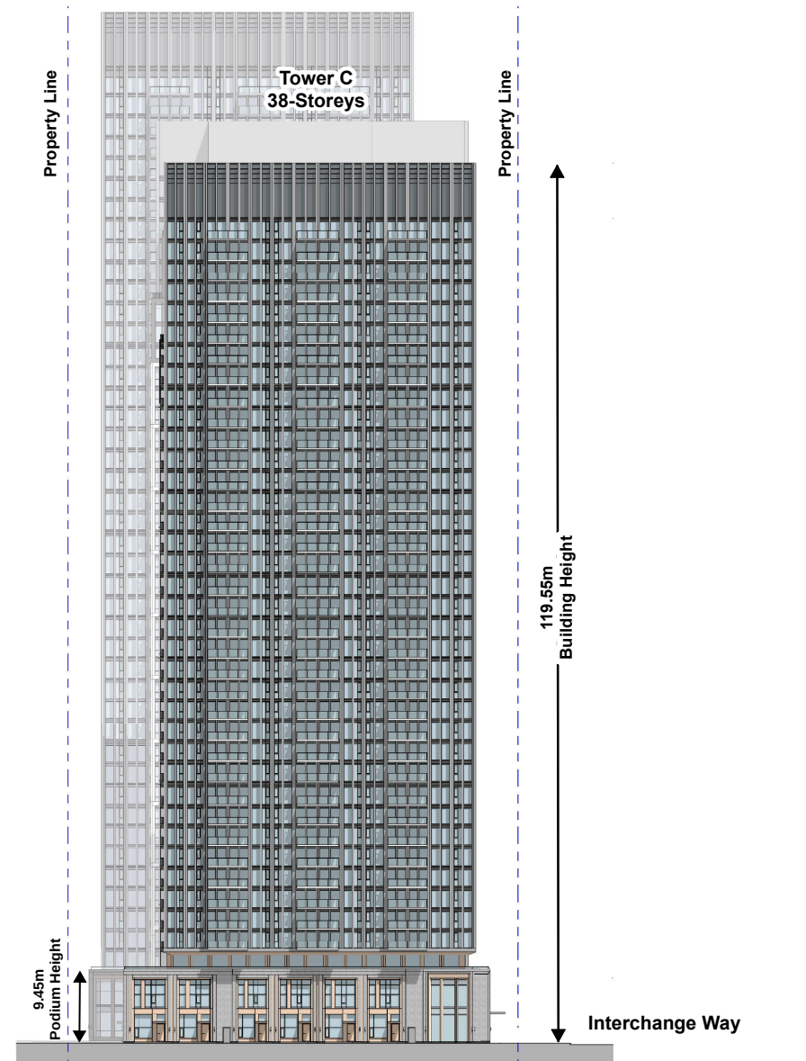
West Elevation - Facing Public Square
