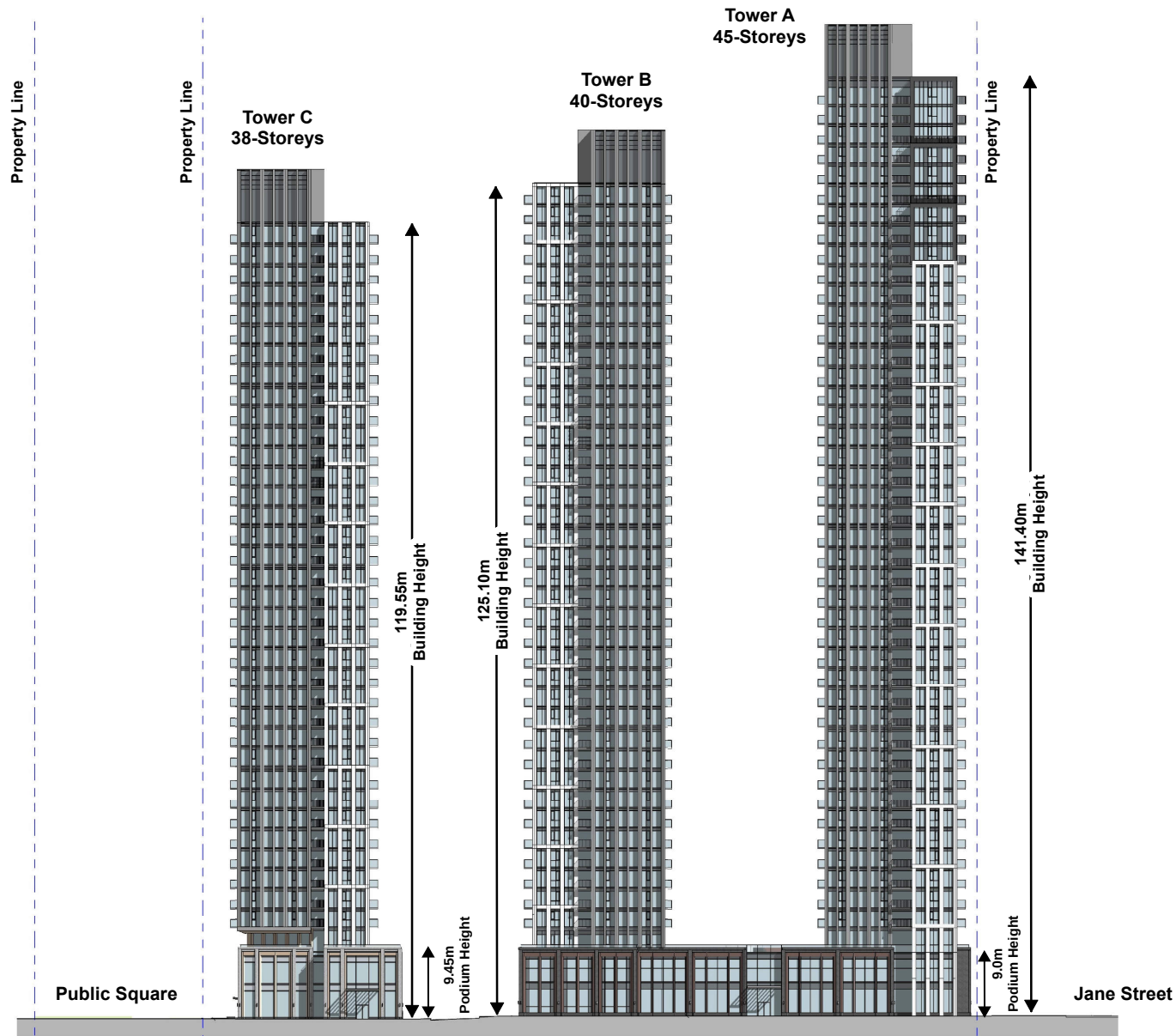
South Elevations - Facing Interchange Way
