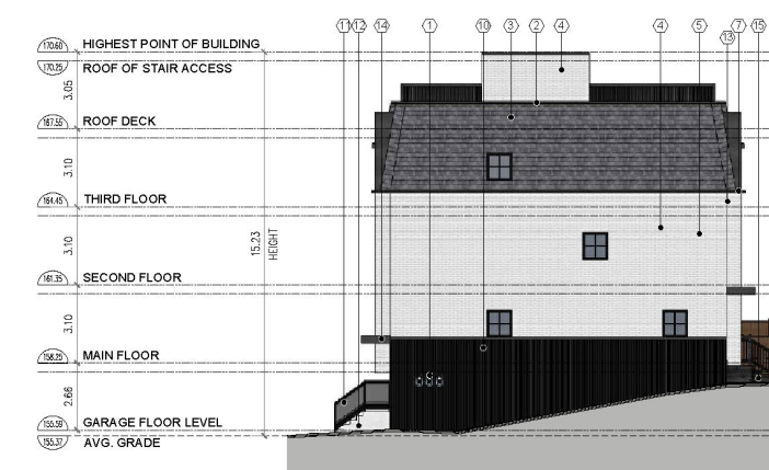
04 TYPE 1 (BLOCKS 4 TO 7) SIDE 2 ELEVATION A301 SCALE: 1:200
