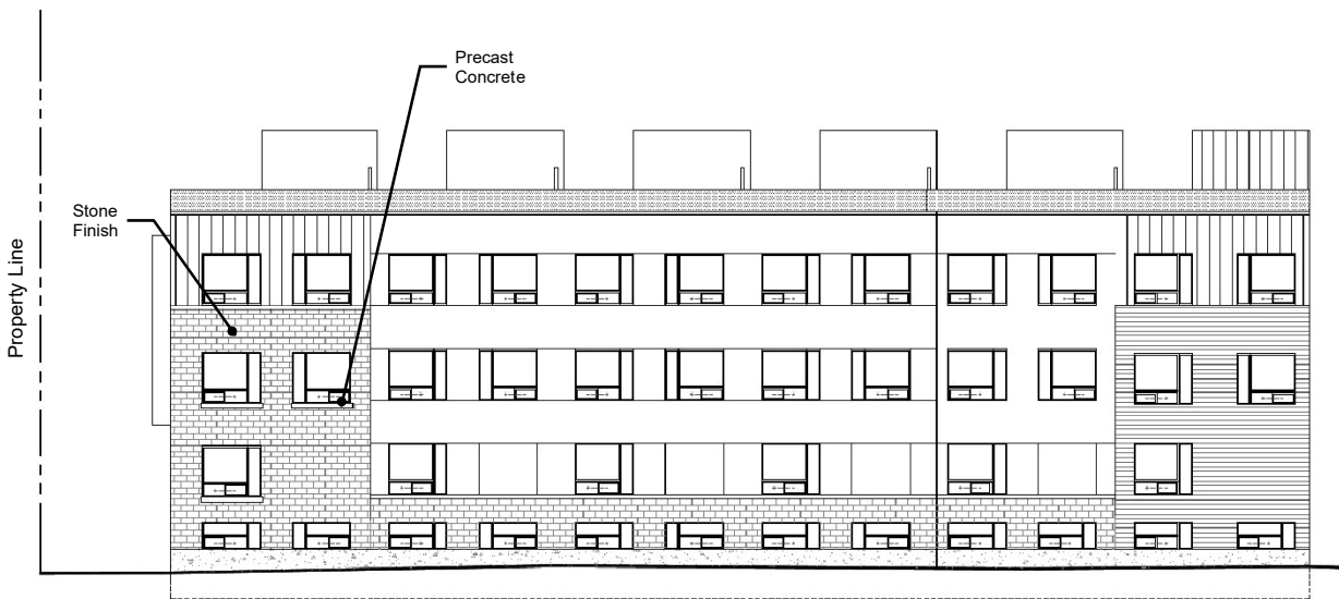
West Elevation
