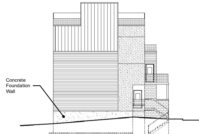
North Elevation
