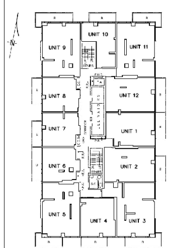
RESIDENTIAL UNITS 1 TO 12, INCLUSIVE, ON LEVELS 20 AND 21
