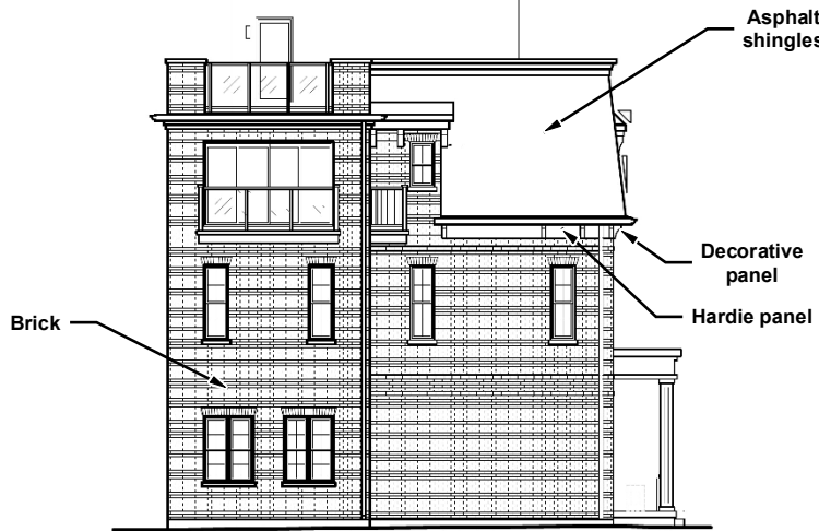
West (Left Side) Elevation - facing Future Private Road
