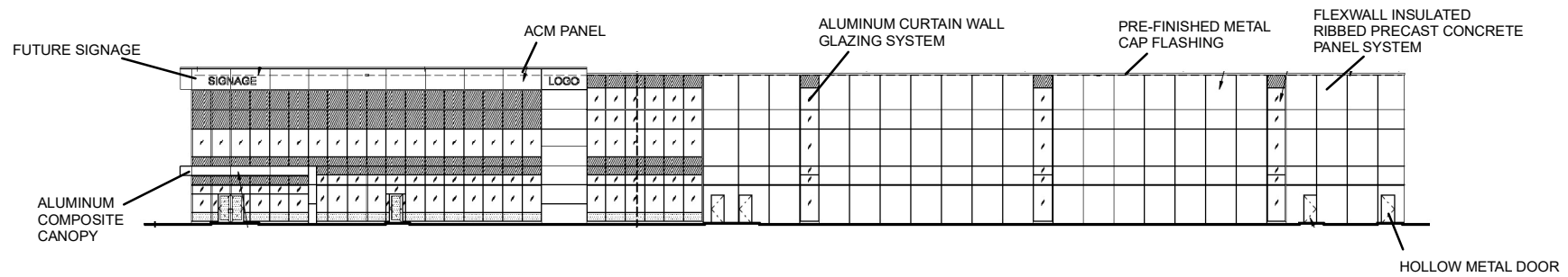
NORTH ELEVATION (FACING KEYES COURT)
