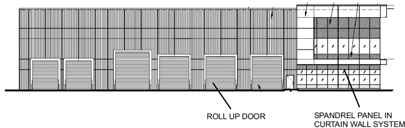
EAST ELEVATION
