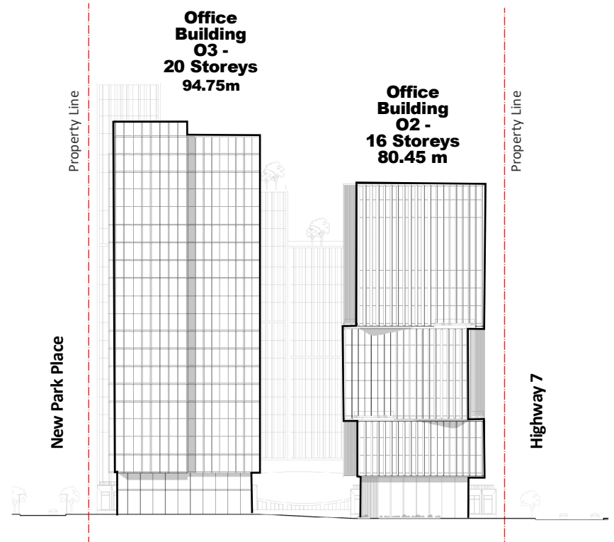
West Elevations
