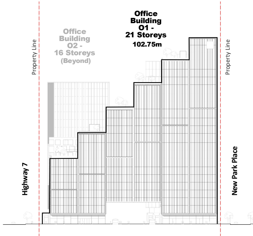
East Elevations
