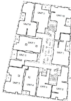
PLAN VIEW ILLUSTRATING UNITS 1 TO 10 INCLUSIVE (Residential) LEVEL 43
