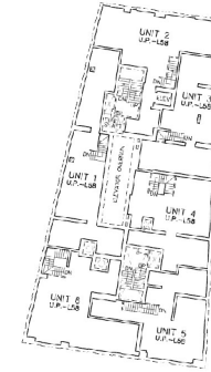
PLAN VIEW ILLUSTRATING LEVEL 59 NO UNITS UPPER PORTION OF UNITS 1 TO 6 INCLUSIVE (Residential), LEVEL 59
