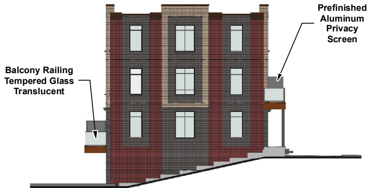
West Elevation
