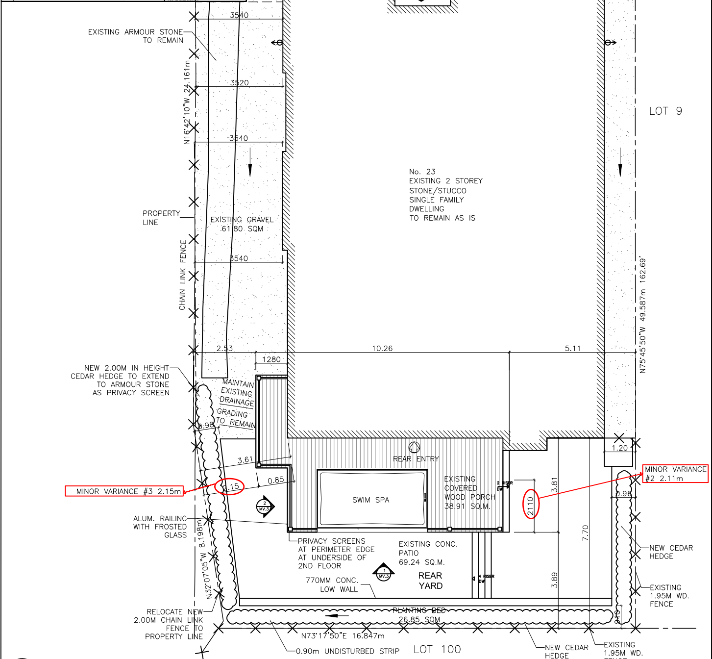
1 PROPOSED SITE PLAN MV.02 SCALE 1:150
