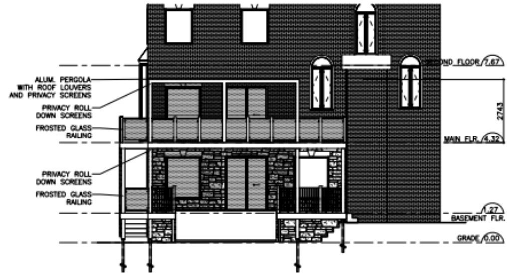
1 PROPOSED REAR ELEVATION MV.03 SCALE 1:150
