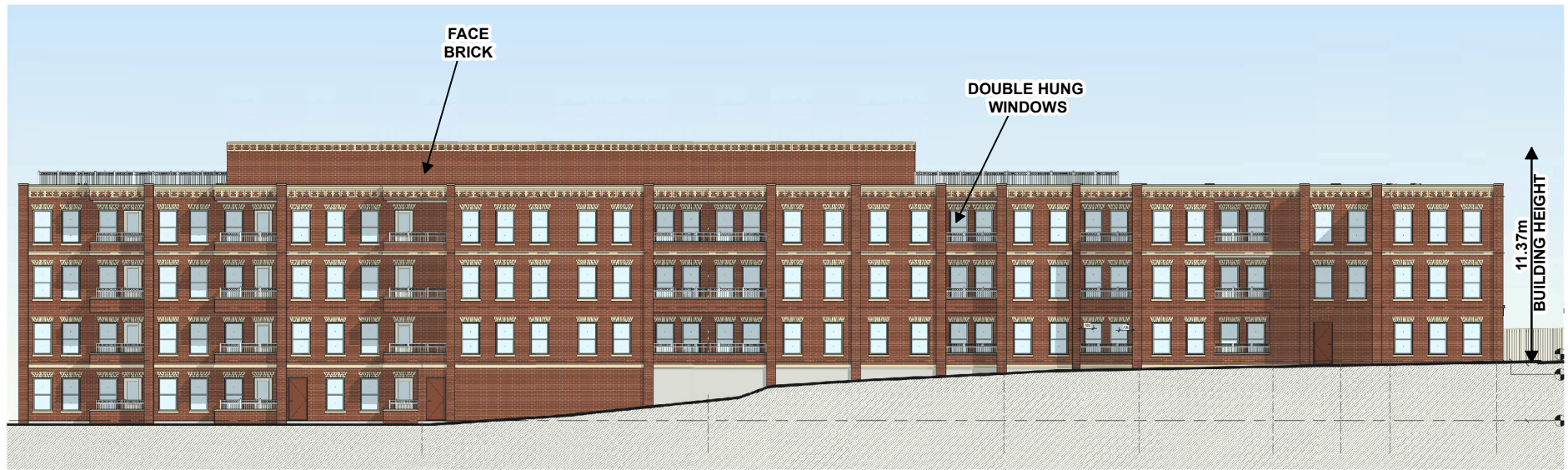
NORTH ELEVATION
