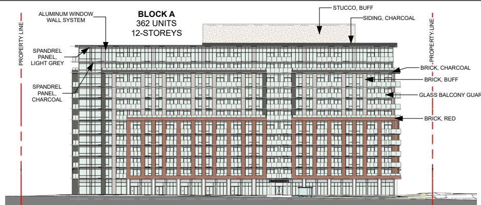
EAST ELEVATION (FACING BATHURST STREET)
