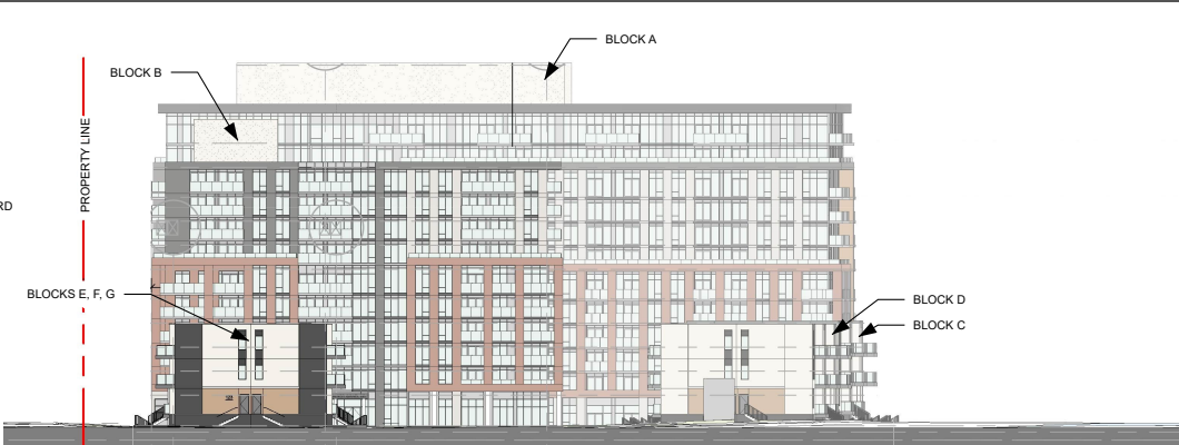
WEST ELEVATION
