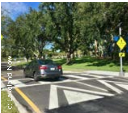
Figure 4.66. Raised crosswalk.
