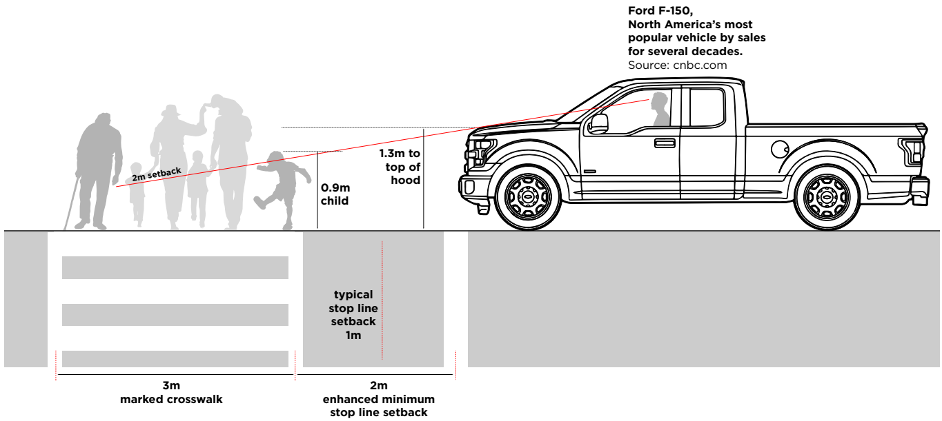
Figure 4.84. Enhanced stop line location improves views of pedestrians at intersections for large design vehicles.
