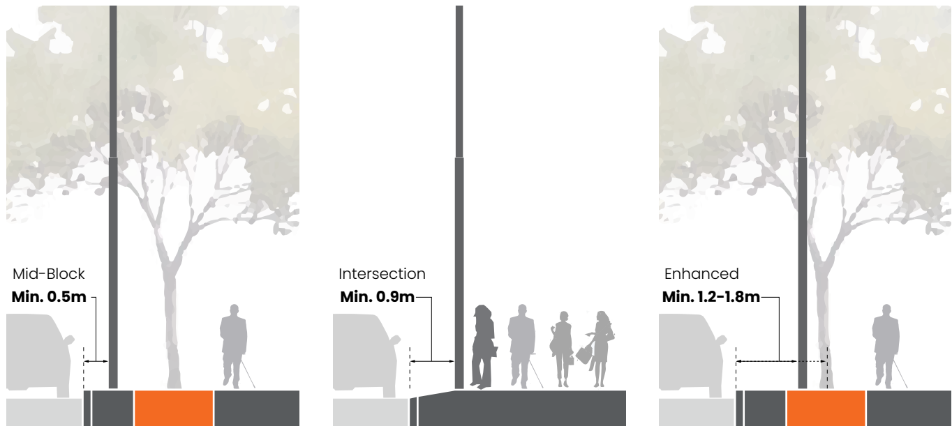
Figure 4.24. Lateral offsets for Vaughan streets, based on TAC 2017 Guidance. All measurements from face of curb. Mid-block: minimum 0.5m; intersections: minimum 0.9m; enhanced offset for Urban Streets where space permits: 1.2m to 1.8m.
