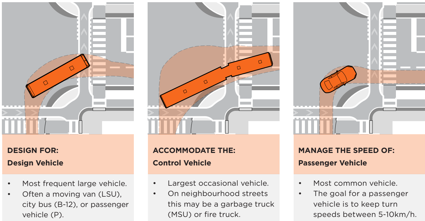
Figure 4.57. Design and control vehicle types to inform turning radii at intersections.
