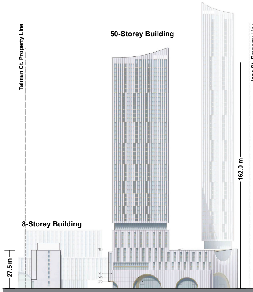
North Elevation
