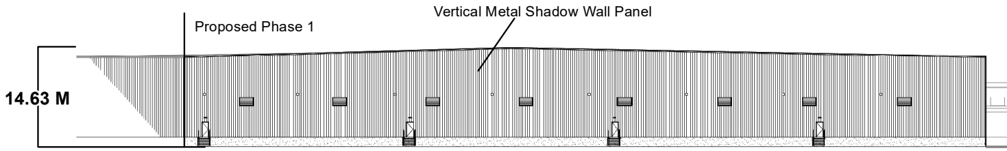
South Elevation Phase 1
