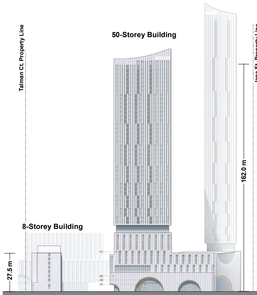
North Elevation
