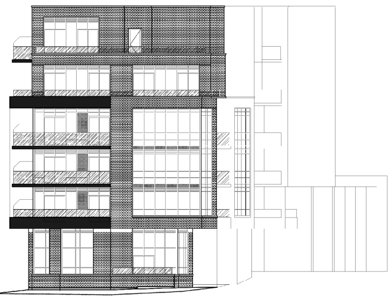
SOUTH ELEVATION
