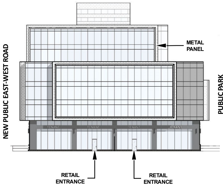
EAST ELEVATION
