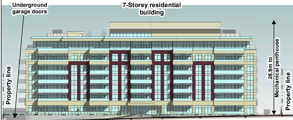
EAST (FRONT) ELEVATION - FACING ISLINGTON AVENUE
