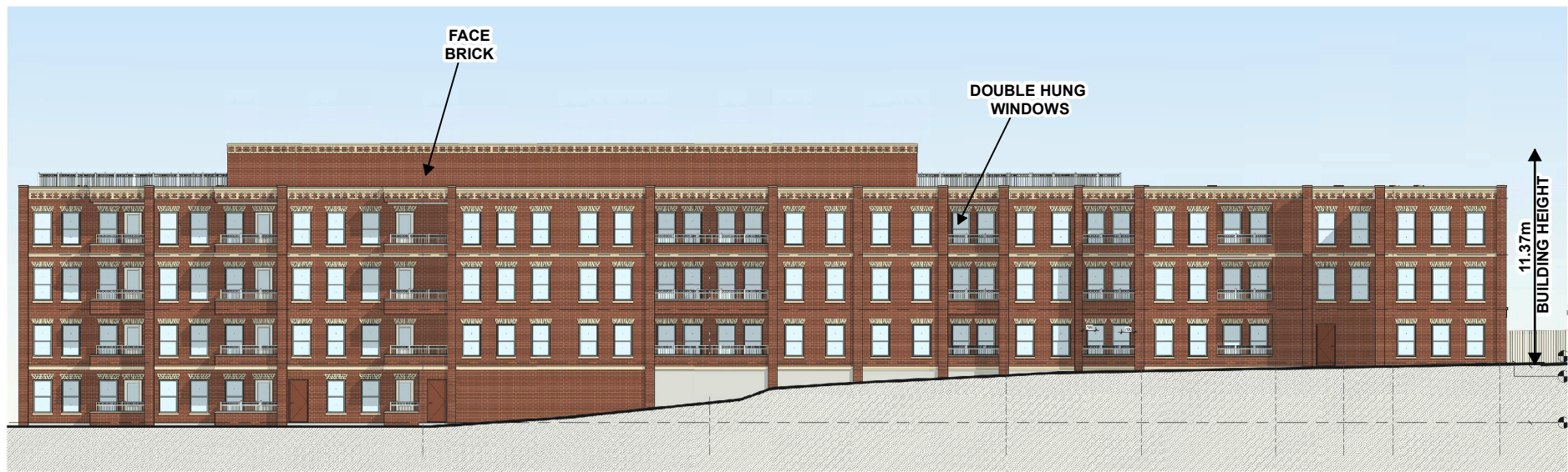
NORTH ELEVATION
