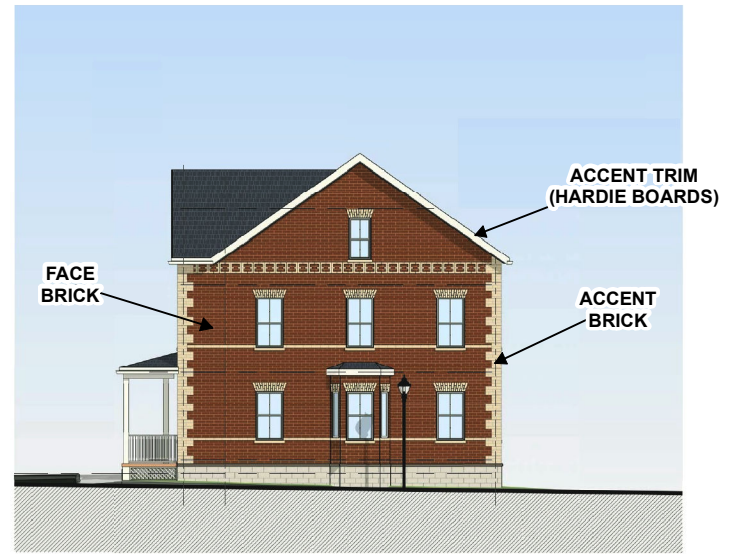
SOUTH ELEVATION
