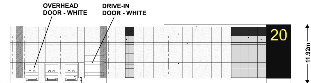
WEST ELEVATION
