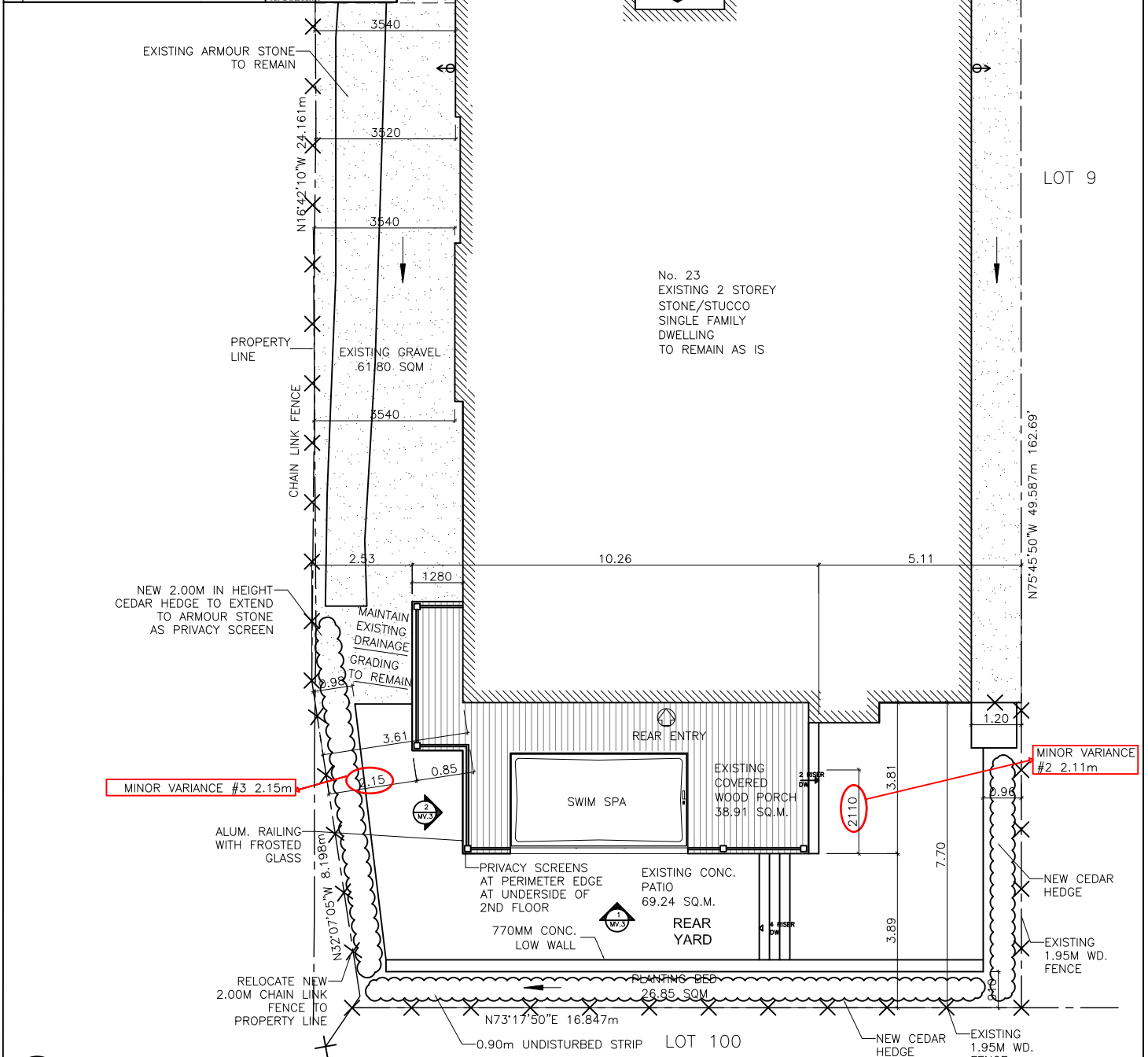
1 PROPOSED SITE PLAN SCALE 1:150
