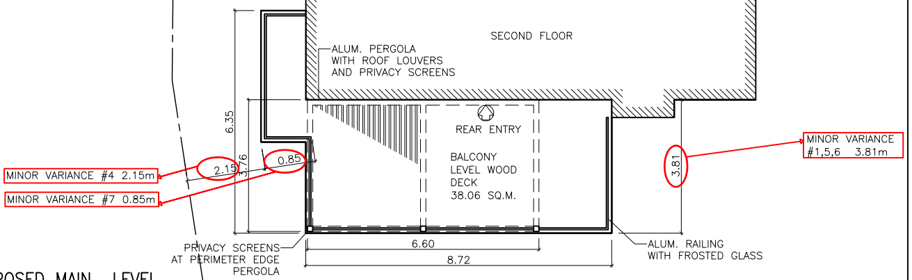
2 PROPOSED MAIN LEVEL SCALE 1:150
